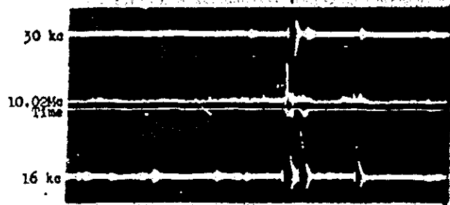
Fig. 3.100 Narrow-band responses Shot No. 7 3400 km from ground zero
